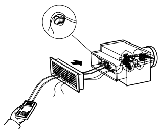
Figure 1. Measurement with two tubes.
