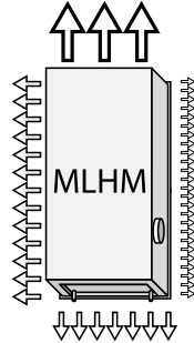
Figure 4. Example of nozzle configuration for a double-mounted unit - MLHM.
