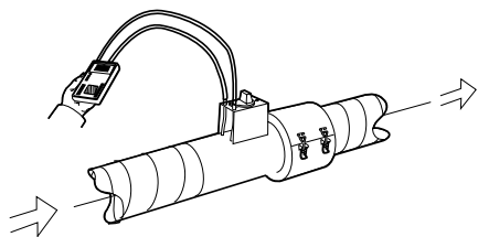
Figure 2. Measurement with two tubes.
