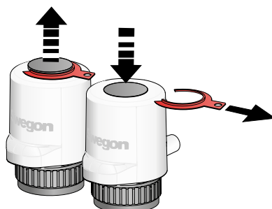
Figure 2. ACTUATOR position indicator
