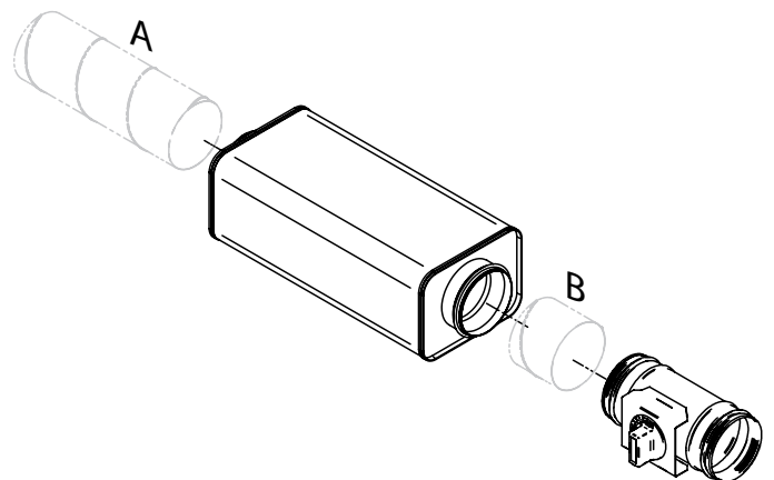
Figure 27. Supply air kit, PARAGON T-SAK-CAV-125 Spiral ducts are not included. Spiral duct A: Min. length: 330mm Spiral duct B: Min. length: 70mm
