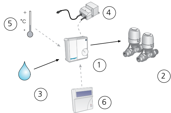
Figure 14. Factory-fitted LUNA control equipment
