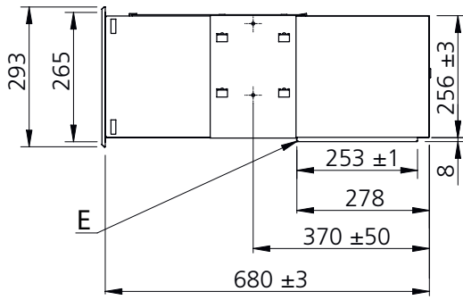
Figure 24. Viewed from end panel
