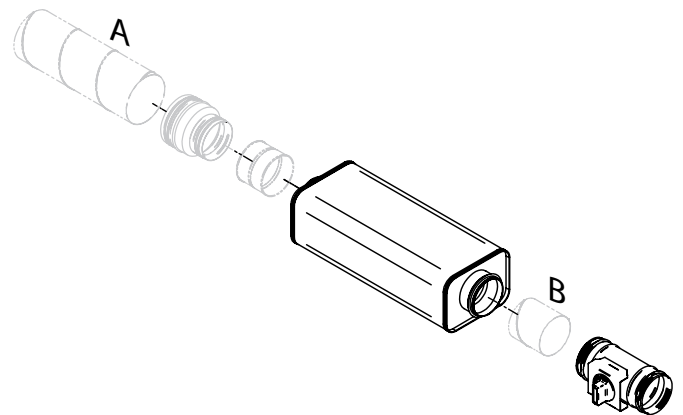
Figure 28. Supply air kit, PARAGON T-SAK-CAV-100 Size 100 spiral ducts and jointing sleeves are not included. Spiral duct A: Min. length: 330mm Spiral duct B: Min. length: 70mm
