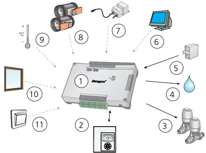
Figure 11. Factory-fitted CONDUCTOR control equipment
