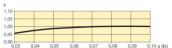
Diagram 2. Water flow – capacity correction
