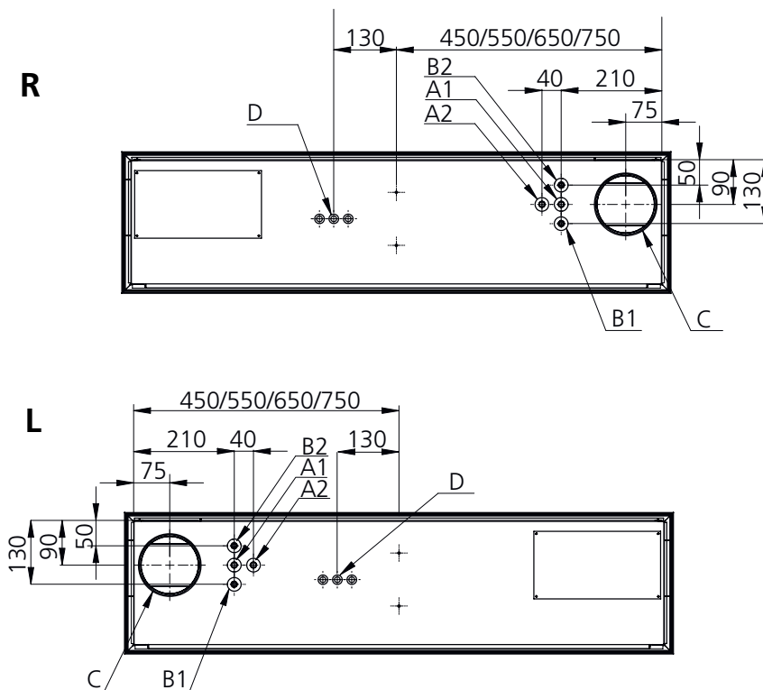
Figure 23. View of the backside, connections L = left-hand connection; R = right-hand connection
