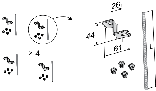
Figure 19. Suspension kit, SYST MS M8
