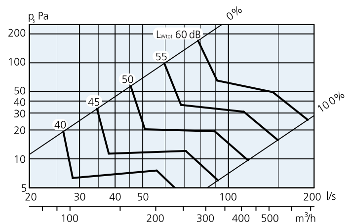
Diagram 9. Commissioning range, SYST CRPc 9-160 damper
