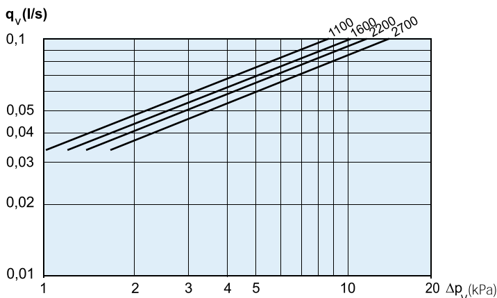
Diagram 5. Pressure drop – water flow, heating
