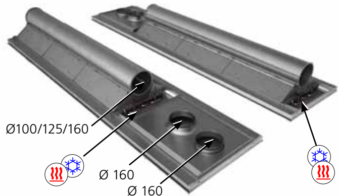
Figure 10. PACIFIC SA/EA with capacity module and additional SA/EA - Ø160 mm, two options for connection points for cooling and heating pipes.
