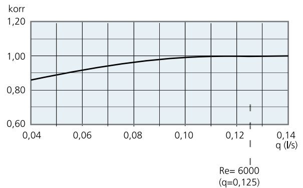
Diagram 3b. Water flow – capacity correction, cooling Length of Capacity module: 2,200 and 2,700 mm
