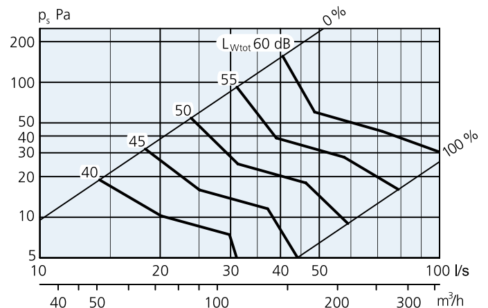
Diagram 8. Commissioning range, SYST CRPc 9-125 damper
