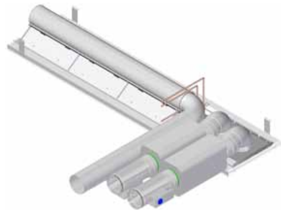
Figure 54. Example with PACIFIC SAE/EA incl. CAV kit with air and water connections from the side.
