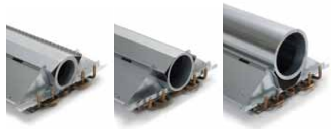
Figure 9. Capacity module - Ø100; Ø125 and Ø160 mm
