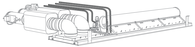
Figure 13. Pacific SA/EA with water pipes connected between the capacity module and the SA/EA module.
