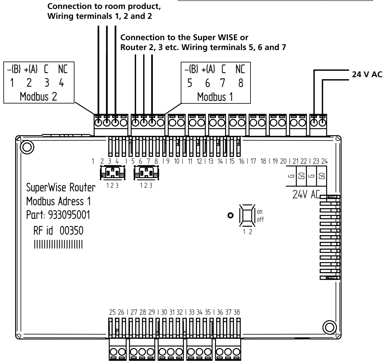
Figure 2. Wiring diagram for the Super WISE Router
