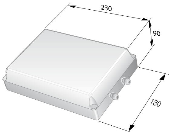
Figure 5. Super WISE Router with enclosure
