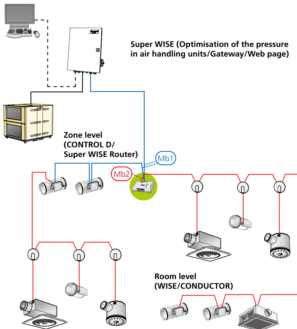
Figure 1. Super WISE Router supersedes zone products in smaller ventilation systems, without requirement for zone control. Zone level: blue line. Room level: red line.
