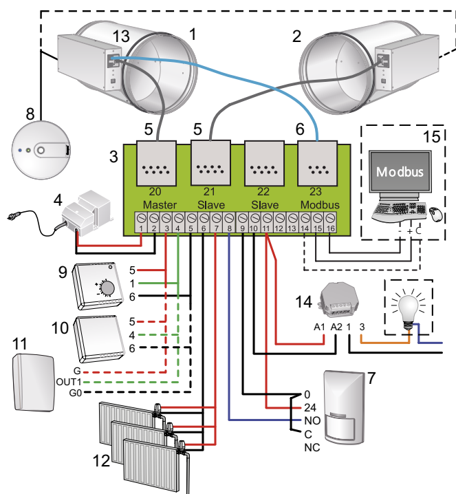
Figure 4. Wiring of master/slave-units and accessories.
