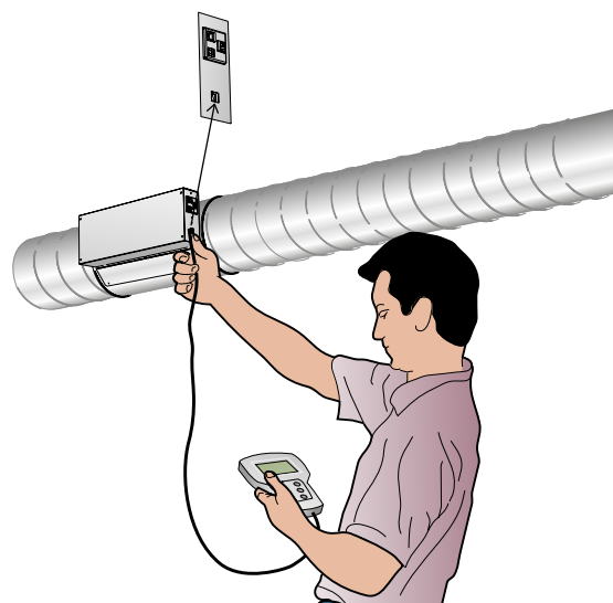
Figure 5. Wiring TUNE Adapt for checking and changing set points. Connection is made directly into the single socket on the side of the damper or the junction box of the extension cable. If DETECT SME is installed, TUNE Adapt is connected to SME instead. Communication with the parent system is disconnected while TUNE Adapt is connected.
