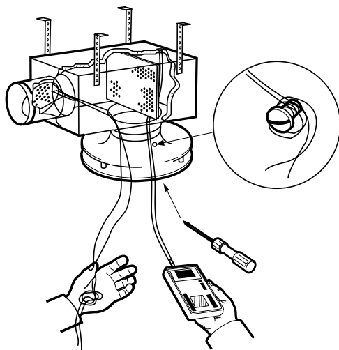
Figure 1. Example ALS, measurement with one tube.
