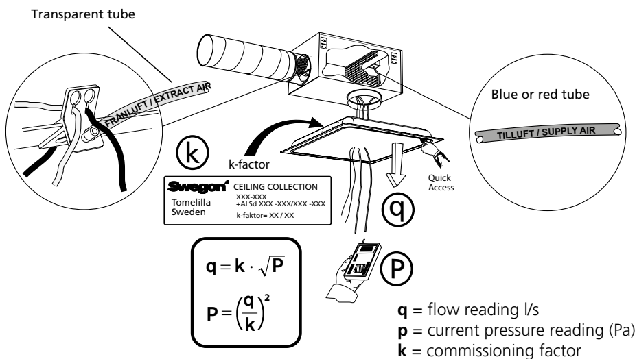
Figure 2. Example ALS, measurement with two tubes, Ceiling Collection.
