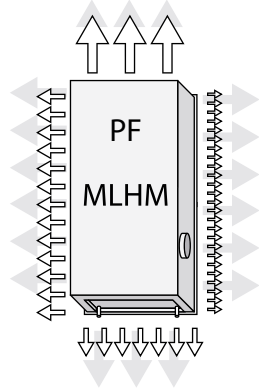
Figure 7. Nozzle setting example PARASOL PF two-module unit - MLHM.
