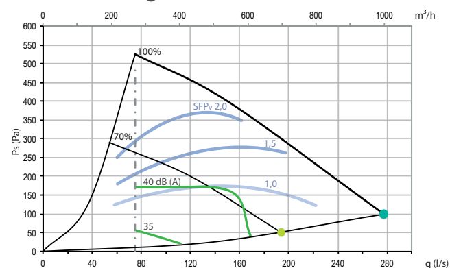
Air volumes and sound power level to surroundings
