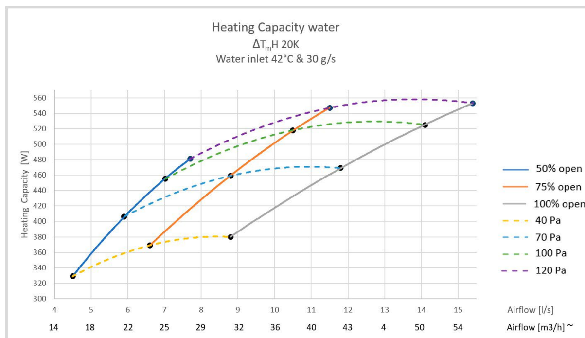
Figure 11. Achieved heating capacity with CASA Climate CCF 600 mm, depending on nozzle setting and nozzle pressure.
