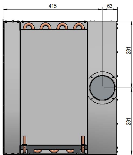
Figure 23. Dimensions CASA Climate CCF 600, air connection side 6. For 1000 length the dimension 281 is instead 481.
