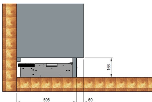
Figure 21. Dimensions - view from the side with CCF mounted in base of 600 cabinet.
