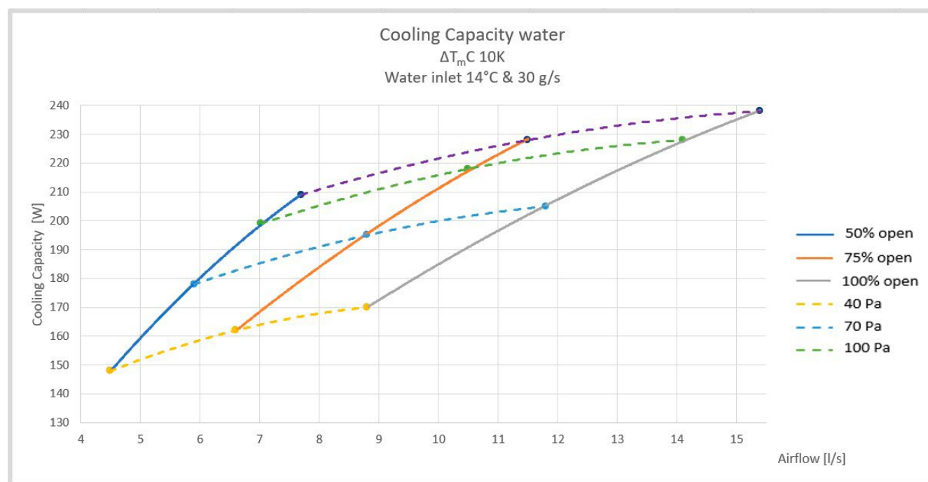
Figure 12. Achieved cooling capacity with CASA Climate CCF 600 mm, depending on nozzle setting and nozzle pressure.
