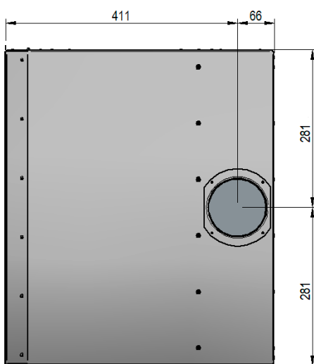
Figure 24. Dimensions CASA Climate CCF 600, air connection side 5. For 1000 length the dimension 281 is instead 481.
