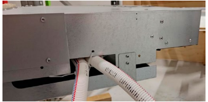
Figure 27. Cut-out for routing the water pipe out from the side of the product.
