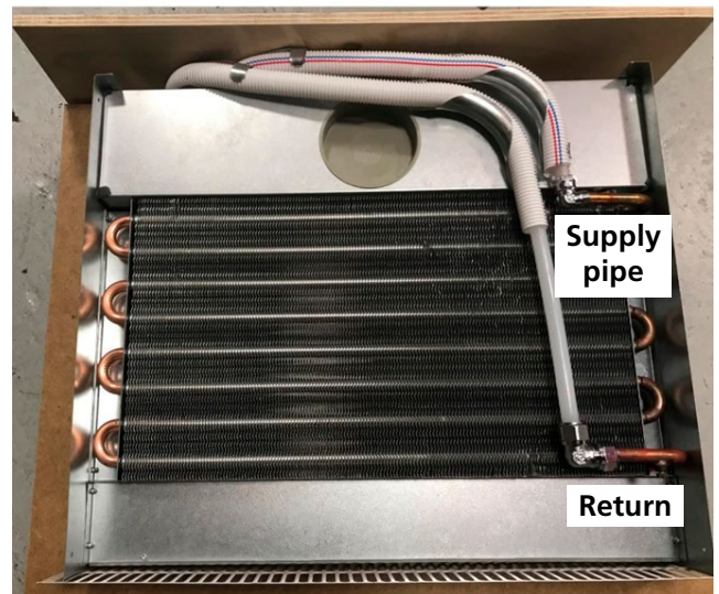
Figure 28. Alternative routing of water pipe, out at the rear of the product.
