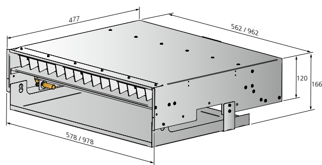
Figure 31. Dimensional drawing excl. grille, incl. leakage indicator, sleeve connection side 2.
