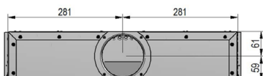
Figure 25. Dimensions CASA Climate CCF 600, air connection side 2. For 1000 length the dimension 281 is instead 481.
