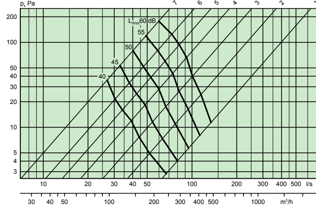
SIRI 160
