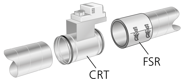
Figur 1. Montering.
