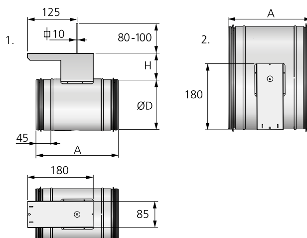
Figur 12. Mått (mm), CRP. 1. CRP-(100-400)-4 2. CRP-(500-630)-4
