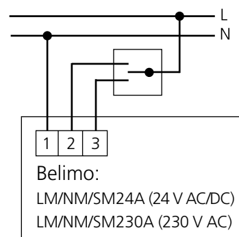
Figure 8. Wiring diagram for Belimo, 3 point regulation.
