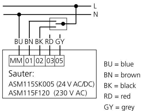
Figure 5. Wiring diagram for Sauter, 3 point regulation.
