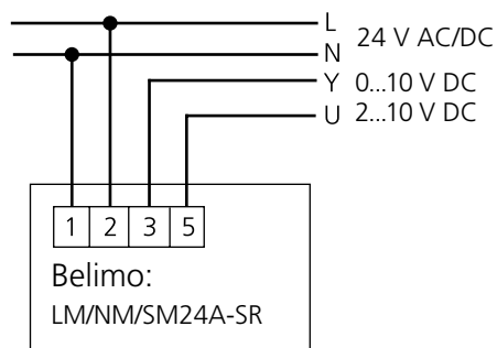
Figure 9. Wiring diagram for Belimo, 0-10 V stepless/modulating regulation.
