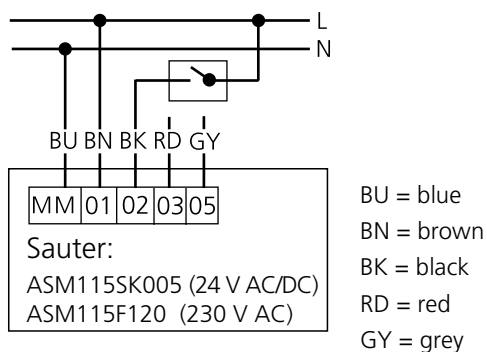
Figure 4. Wiring diagram for Sauter, 2 point regulation.
