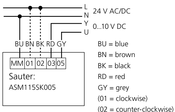
Figure 6. Wiring diagram for Sauter, 0-10 V stepless/modulating regulation.
