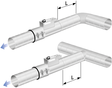
Figure 2. Straight duct length demands, see table.
