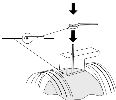
Figur 3. Montering vred CRTT-1
