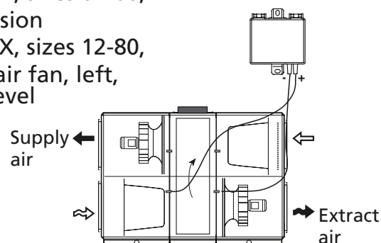
GOLD RX, sizes 04-08, split version GOLD RX, sizes 12-80, Supply air fan, right, lower level
