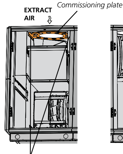
Mounting screws (3 in total)
