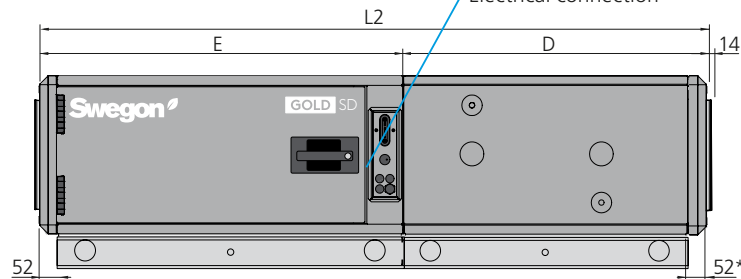
Fan + coil heat exchanger
