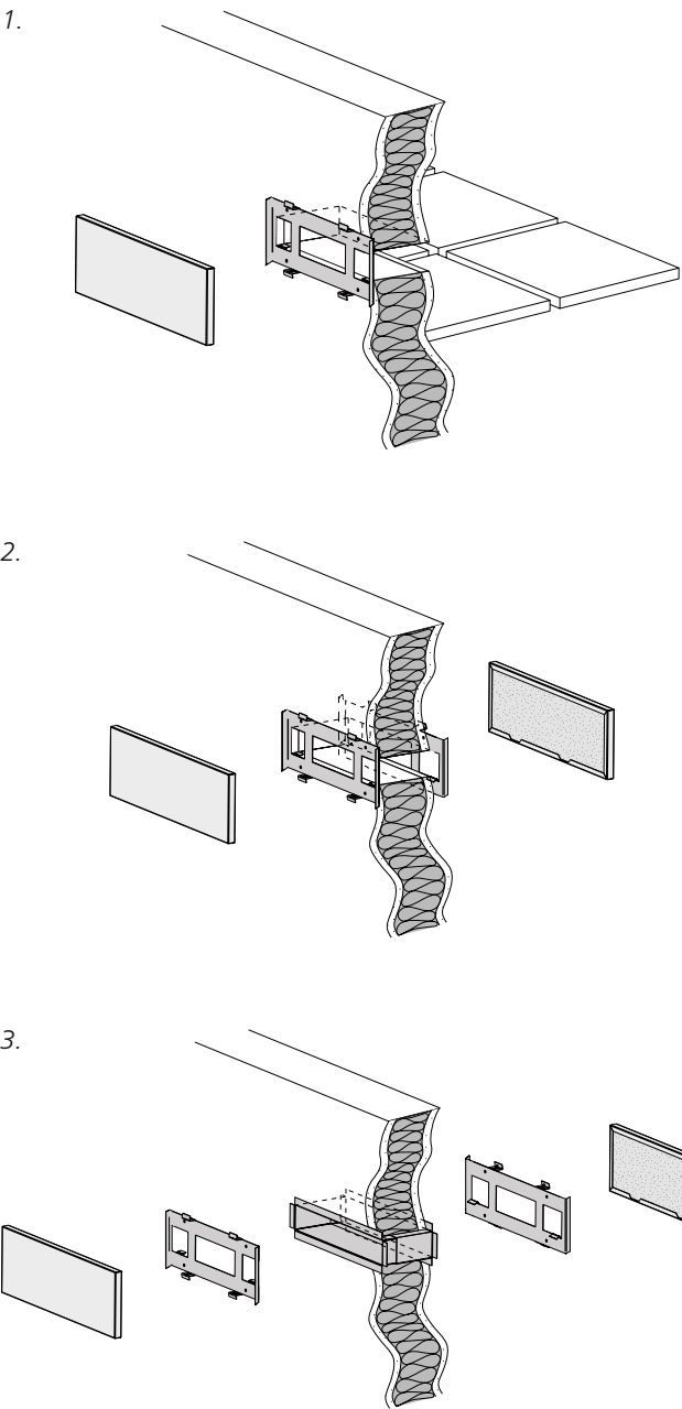
Figure 2. Application options. 1. Concealed installation towards a corridor. 2. Visible installation towards a corridor. Double ORTO. 3. As in (2), but with VGR wall sleeve.
