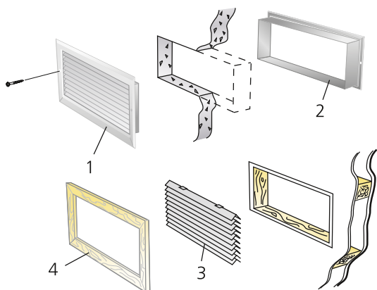
Figur 1. Montering.
