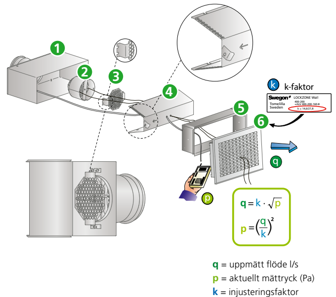
Figur 1. Montering, injustering.
