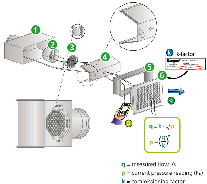
Figure 1. Installation, commissioning.
