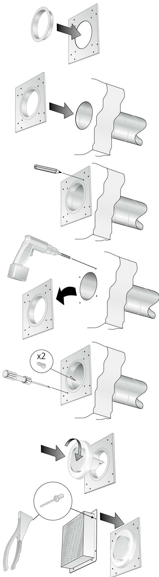
Figure 1. Installation.
