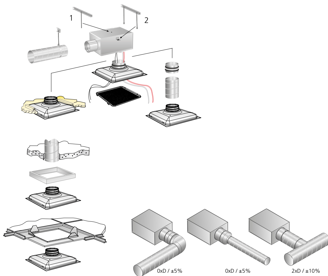
Figure 2. Installation alternatives.
