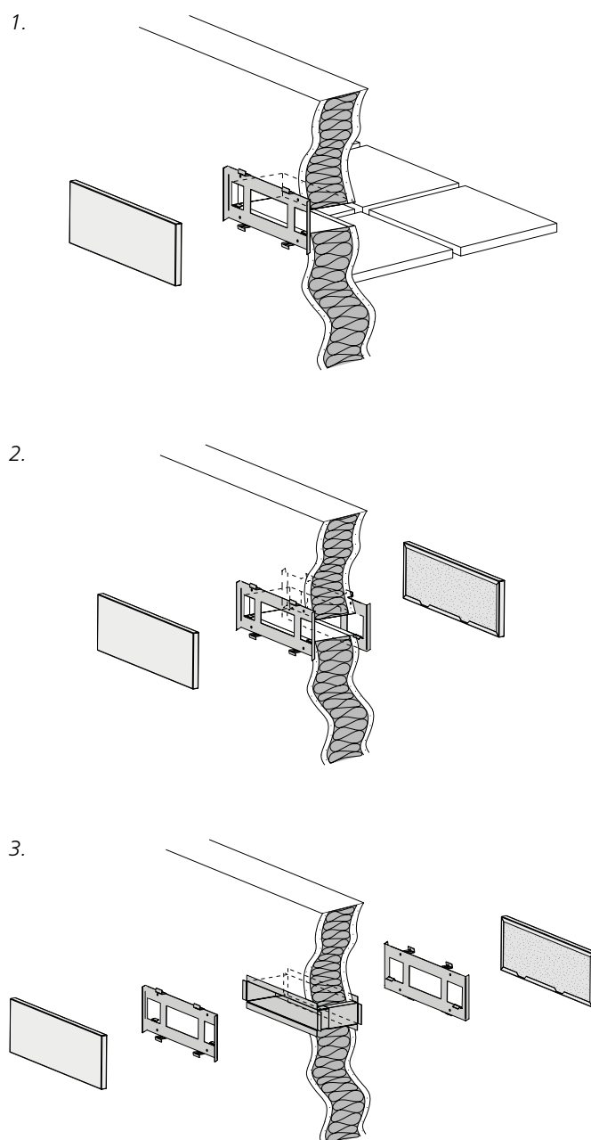
Figure 2. Application options.
