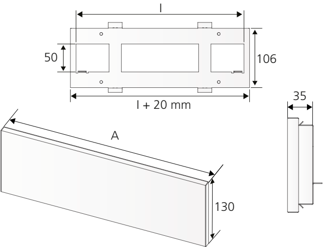
Figure 4. ORTO, dimensions.
