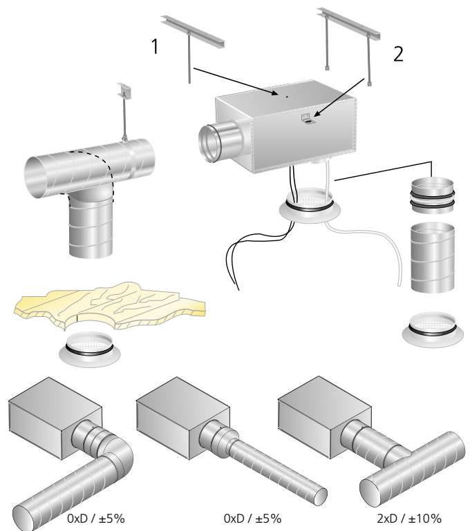
Figur 1. Montering.
