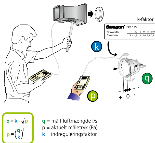
Figur 3. Indregulering.
