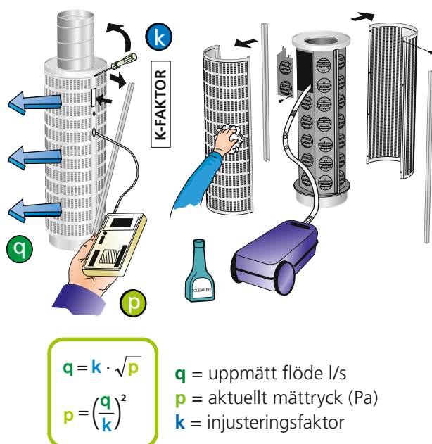
Figur 4. Injustering. Skötsel.
