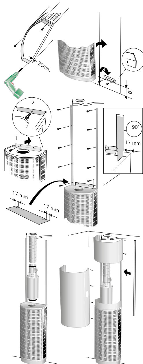
Figur 1. Montering.
