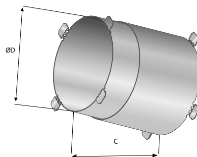
Figure 5. VGC, dimensions.
