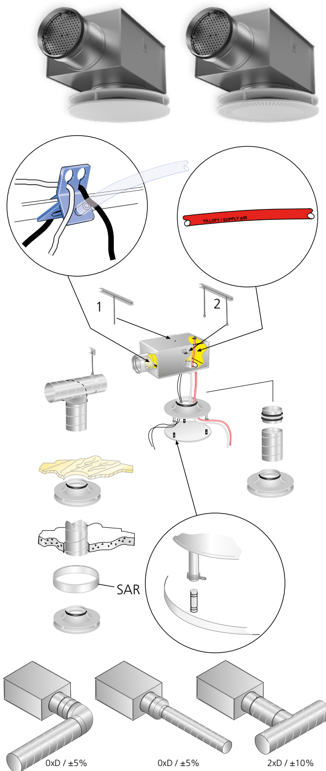
Figure 1. Montage. Innregulering.
