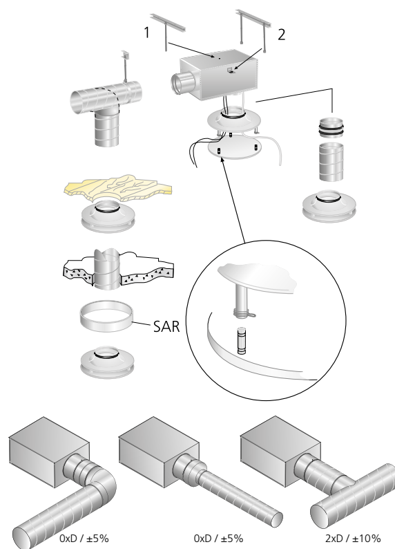
Figure 2. Installation
