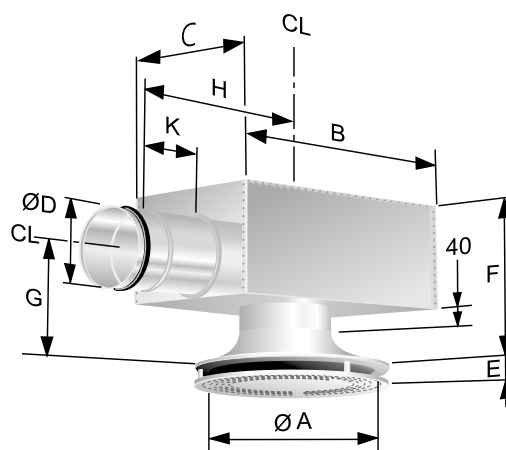
Figure 4. CDK/CKP + ALS. CL = Centerline.
