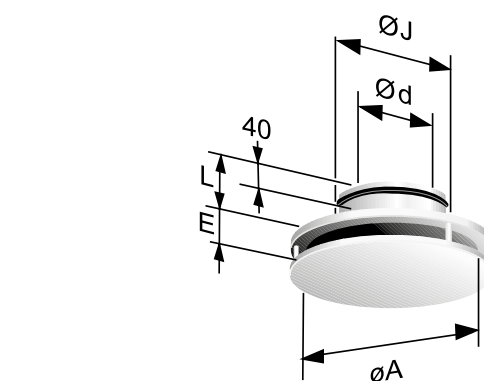
Figure 3. CDK/CKP.
