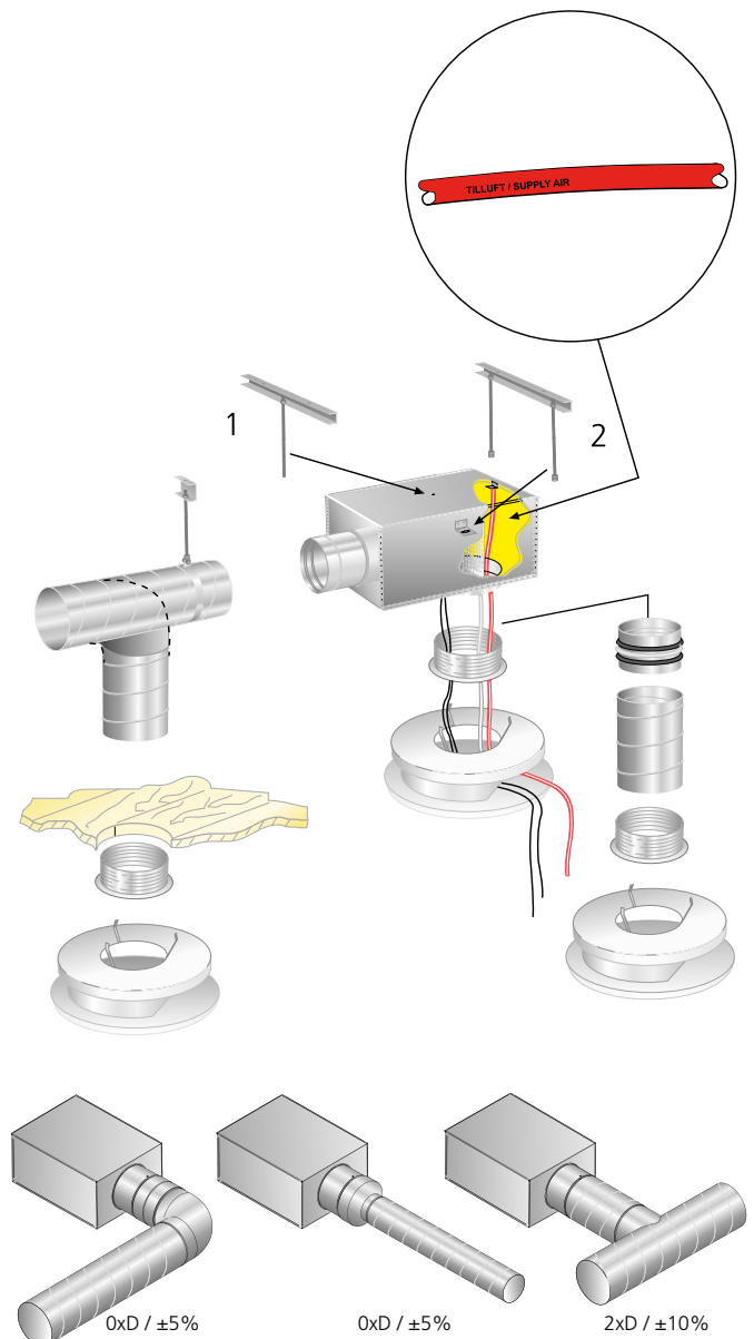
Figur 1. Montering. Injustering.
