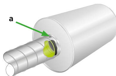
Figure 1. For reasons of safety, connect the connection duct to the raised sheet-metal edge that is fastened inside the connection spigot using screws or pop rivets (a).
