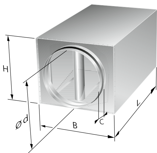
Figure 3. CLA-B – Dimensions
