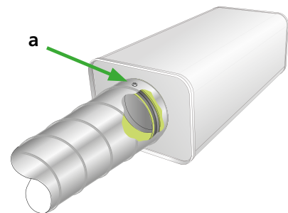
Figure 1. For reasons of safety, connect the connection duct to the raised sheet-metal edge that is fastened inside the connection spigot using screws or pop rivets (a).
