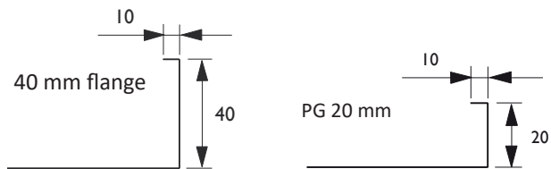
Duct connection
