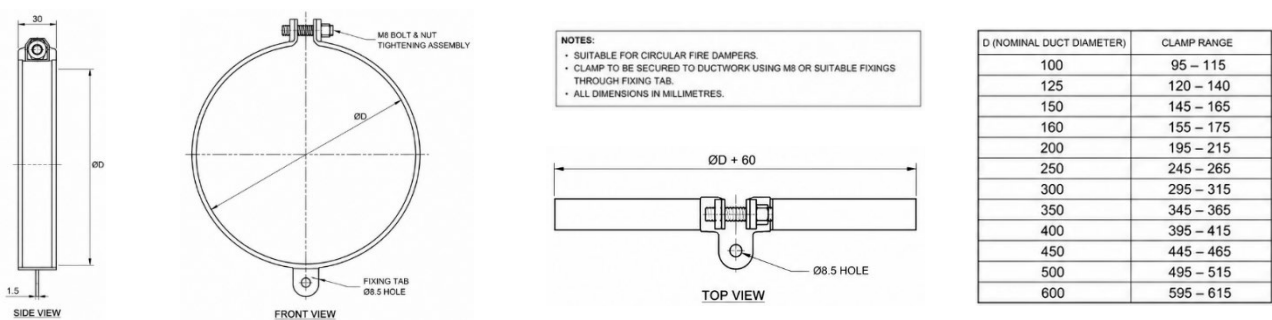
IMAGE OF DUCT CLAMP, DROP ROD GUIDANCE BELOW
