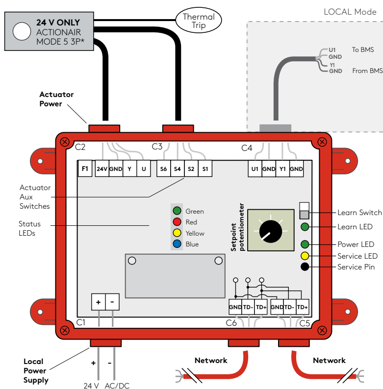
Figure 9. 3P-SFDI-MIFT 24 V Wiring.
