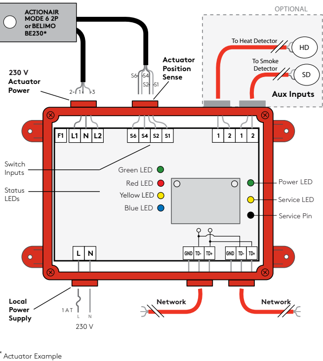
Figure 7. SDI-M/FT 230V Wiring.
