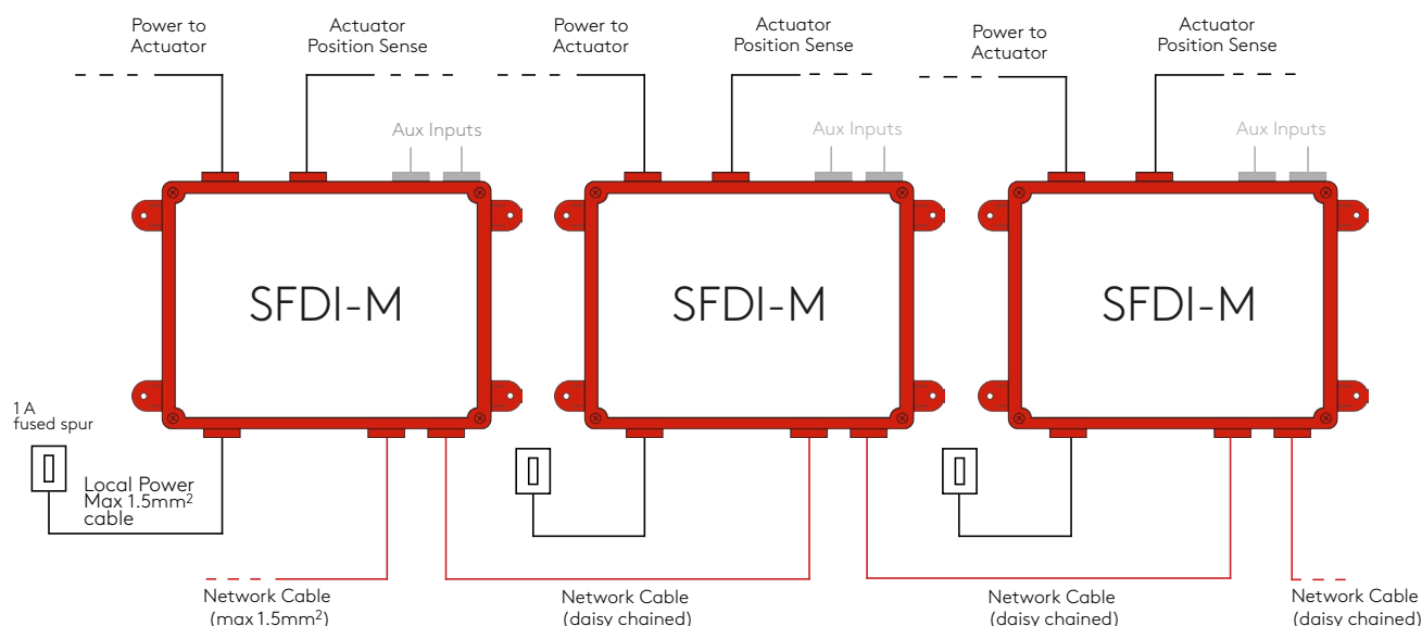
Figure 14. Field Networking Diagram Example - SFDI-Ms.
