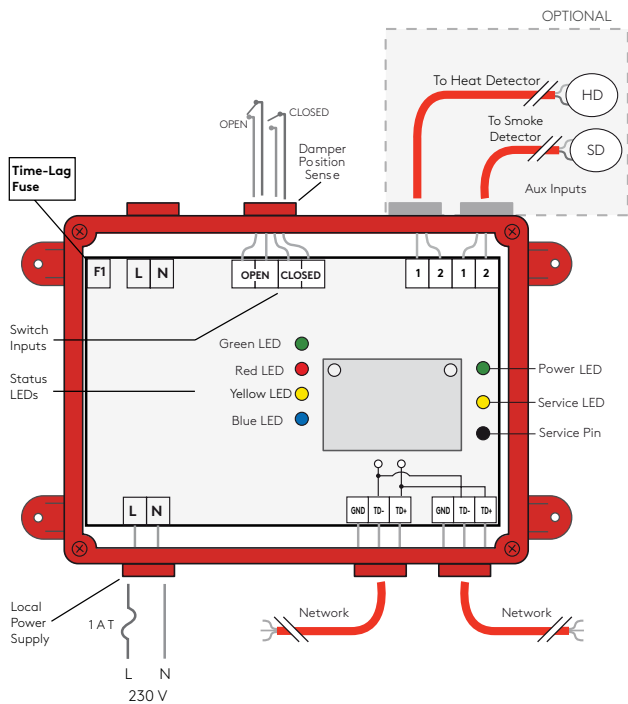
Figure 15. FDI-M/FT 230 V Fuse.
