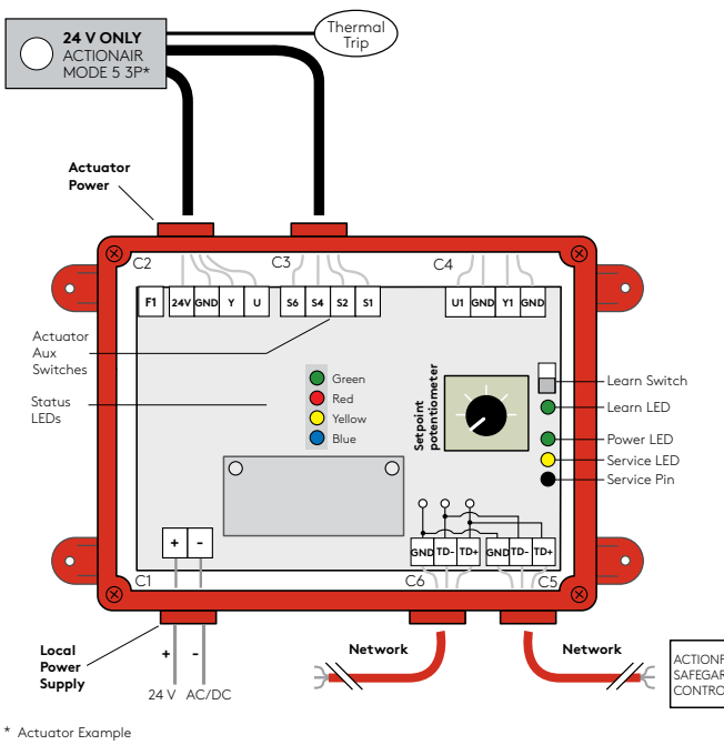
Figure 11. 3P-SFDI-M/FT 24 V Learn Mode.
