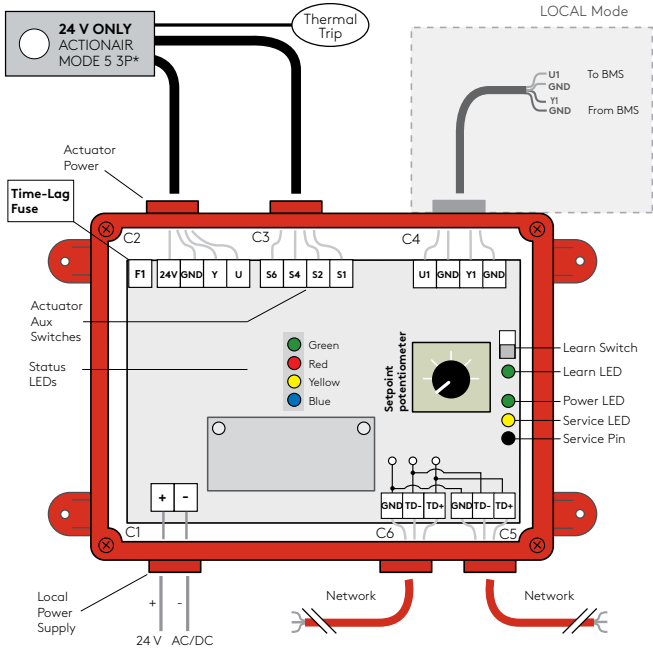
Figure 16. 3P-SFDI-M/FT 24 V Fuse.
