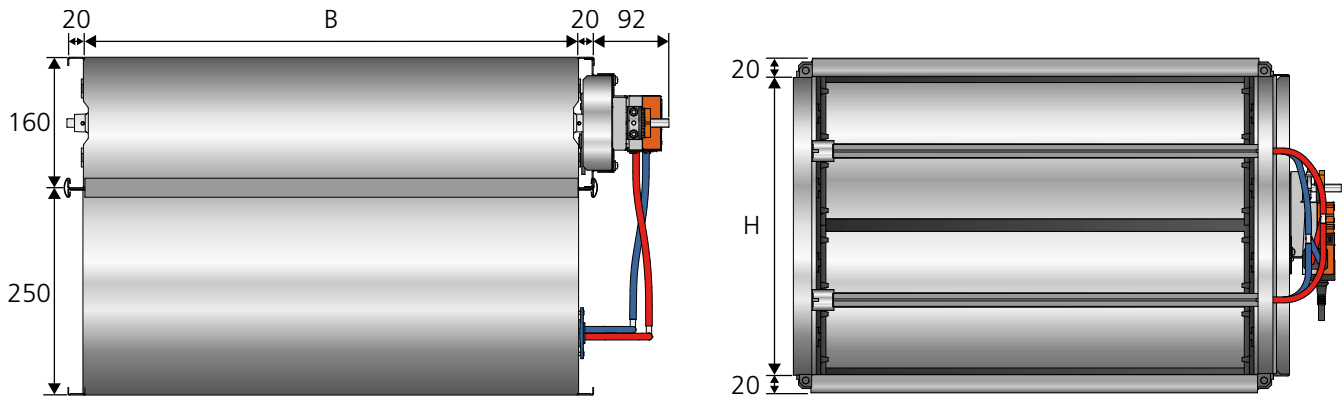
Figure 7. Dimensions (mm), REACT V BMB rectangulaire.
