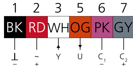
Figure 2. Raccordement.
