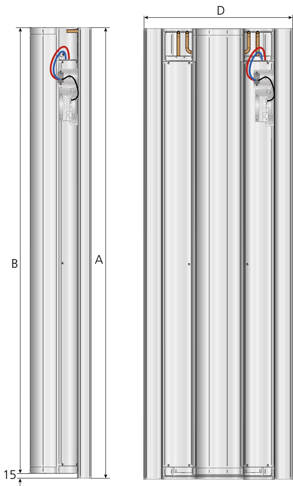
Figure 13. Dimension sketch - full size
