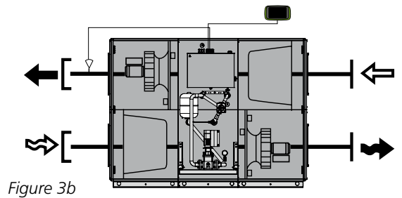
Left-hand version fan arrangement 1
