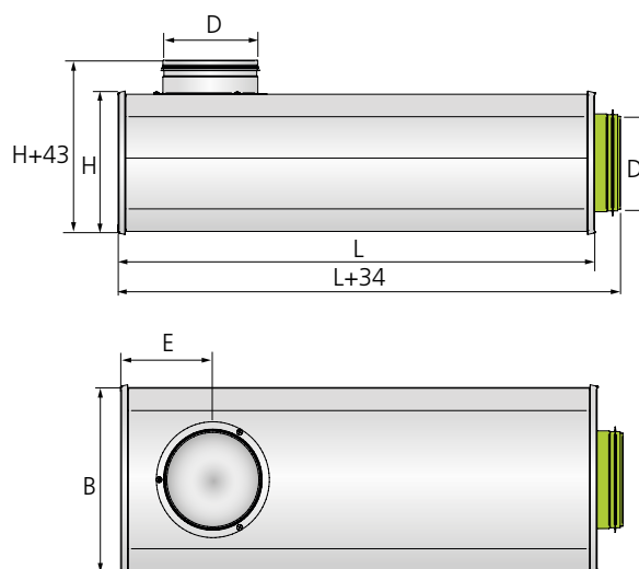
Figure 4. CLV – dimensional drawing (side view)
