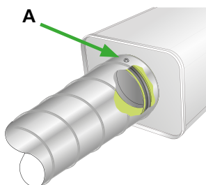
Figure 1. Fasten the connection duct to the turned up sheet-metal edge that is fixed in place inside the connection spigot with a screw or blind rivet (a).
