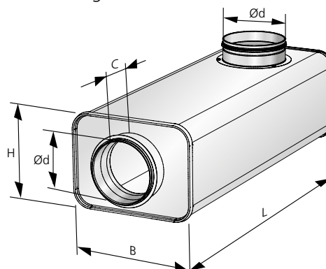
Figure 3. CLV – dimensional drawing
