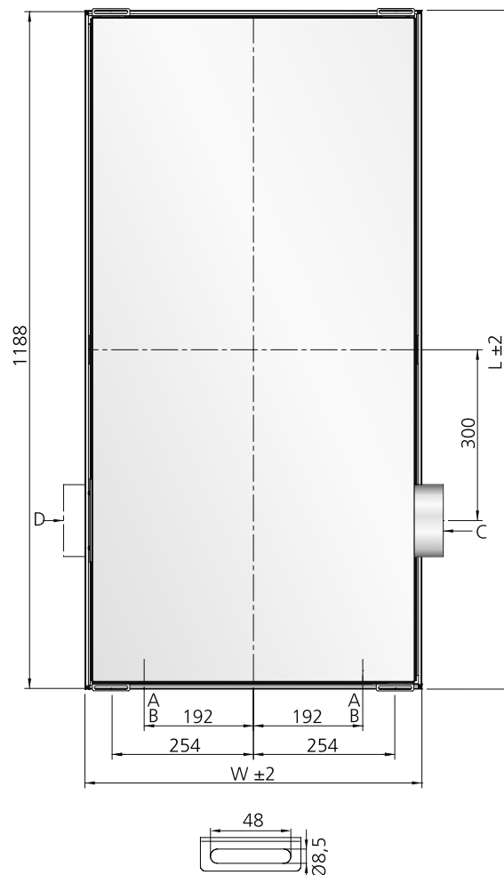
Figur 28. Parasol 1200, toppvy
