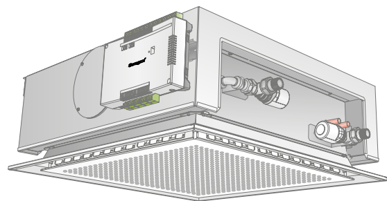
Figur 13. Fabriksmonterad styr - CONDUCTOR (PARASOL c T-COND-XX)
