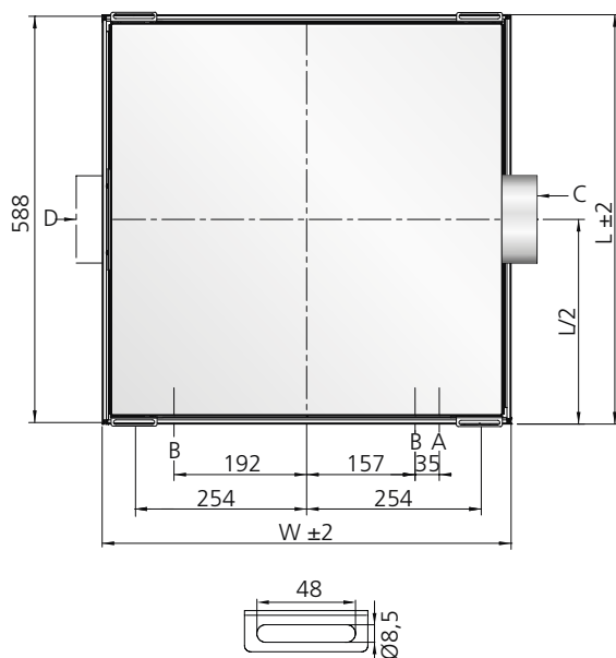
Figur 26. Parasol 600, toppvy
