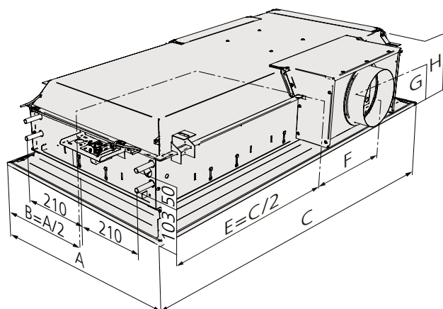
Figure 26. Dimensional drawing - long side connection (the length 1200 with air connection on side 2 is shown in the example).
