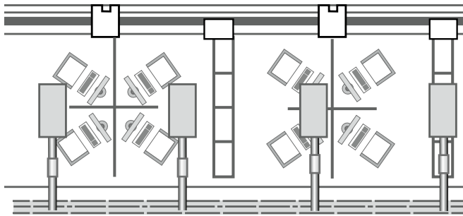
Figure 14. Installation example.
