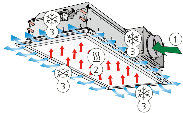
Figure 2. Variant A: Cooling and supply air function
