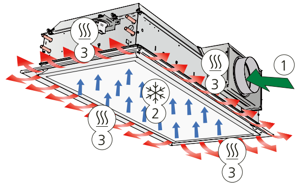
Figure 3. Variant B: Heating and supply air function
