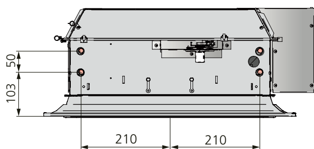
Figure 23. Dimensions, water connection length 600, 1200, 1800
