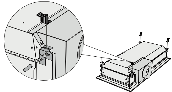
Figure 19. Suspension in four brackets with SYST MS M8
