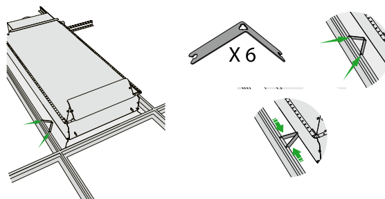
Figure 25. Kit de centrage, SYST CENTERING KIT PARASOL
