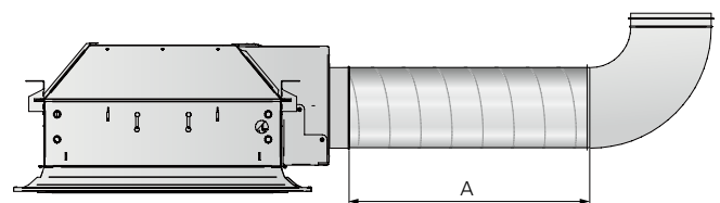
Figure 29. Dimensional drawing, long side connection with bend
