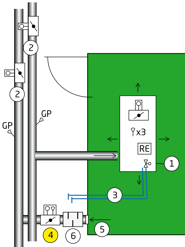
Figure 11. The type room shows PARASOL Zenith AWC in an office Supply and extract air in balance.
