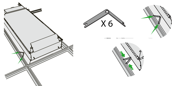
Figure 25. Centring kit SYST CENTRING KIT PARASOL
