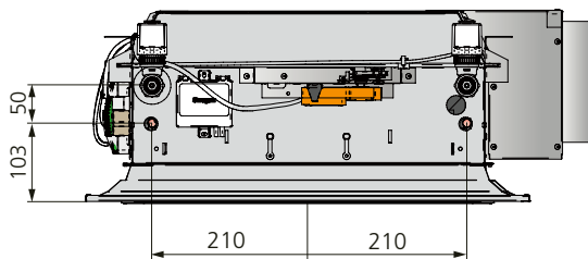
Figure 27. Dimensions, water connection length 600, 1200, 1800
