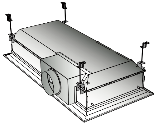
Figure 22. Suspension double-module units
