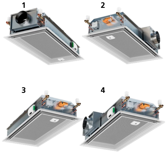
Figure 20. Air connection on side 1 2, 3 and 4
