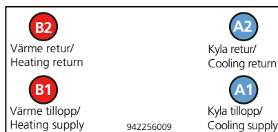
Figure 28. Water connection - Length 600, 1200 and 1800*
