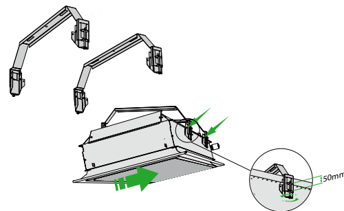
Figure 24. Installation with quick bracket PARASOL Z QUICK SUSPENSION KIT
