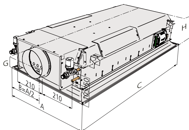
Figure 31. Dimensional drawing - short side connection (the length 1200 with air connection on side 1 is shown in the example).
