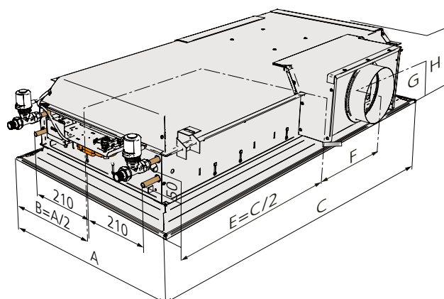
Figure 30. Dimensional drawing - long side connection (the length 1200 with air connection on side 2 is shown in the example).
