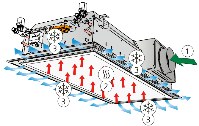
Figure 3. Variant A: Cooling and supply air function
