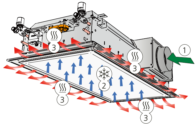
Figure 4. Variant B: Heating and supply air function (also includes cooling function)
