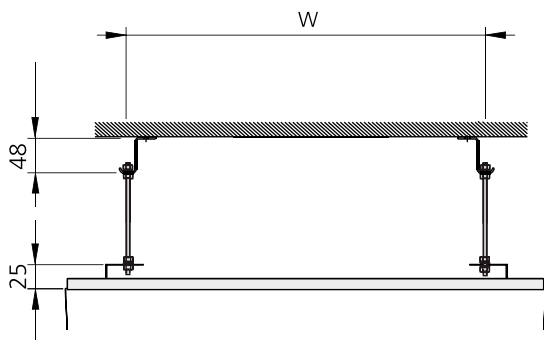
Figura 11. Raccorderia SYST MS.
