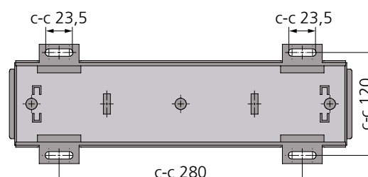
Figure 25. Dimensions - ADRIATIC d T-MD-4S
