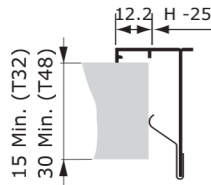
Frame: R16 / R25 / R32 Mounting: CF
