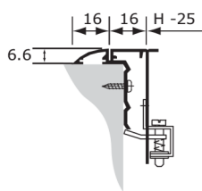
Frame: R16 Mounting: RCHS
