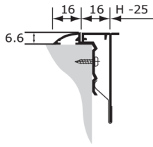
Frame: R16 Mounting: RCCF
