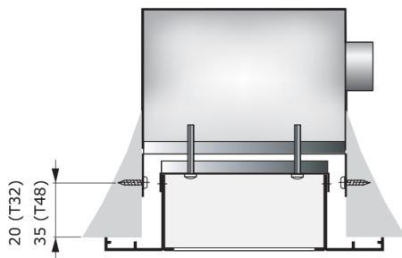
BSSBP (R16 / R25 / R32) Plenum fixing (-15mm)
