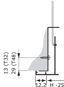
Frame: R25 Mounting: AFVS
