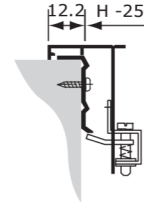
Frame: R25 / R32 Mounting: AFHS
